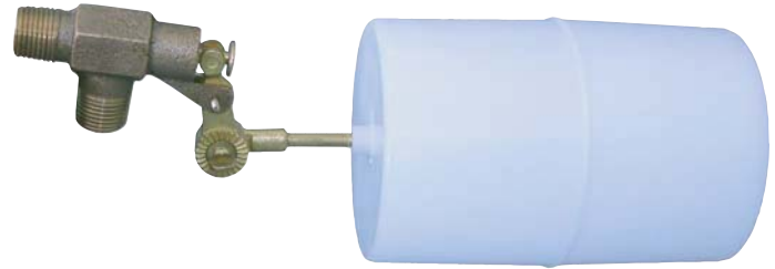
SB119 UPC 7-74996 05303-5 1/2" Brass Valve Assembly Approx. water flow, 5 Gal/min. For SBEE50NG, SBEE100NG, SB351NG, SB352NG, SB354NG
