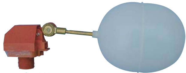
SB118 UPC 7-74996 02032-7 Plastic Valve & Float Assembly 37 litres/minute @ 50 PSI Old style superbowl valve
