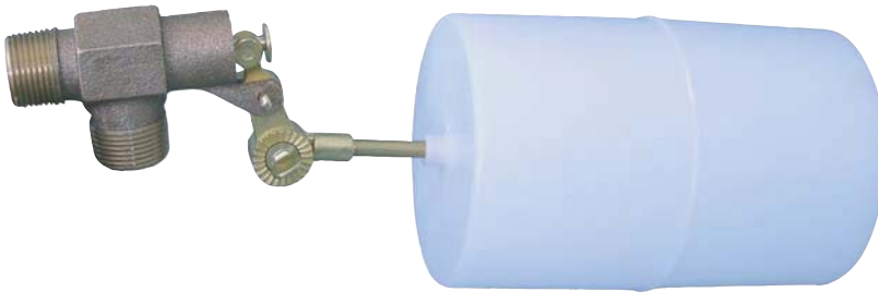
SB120 UPC 7-74996 05304-2 3/4" Brass Valve Assembly Approx. water flow, 10 Gal/min. Will fit old style superbows 4X1, 4X2, 4X4, SB351, SB352
